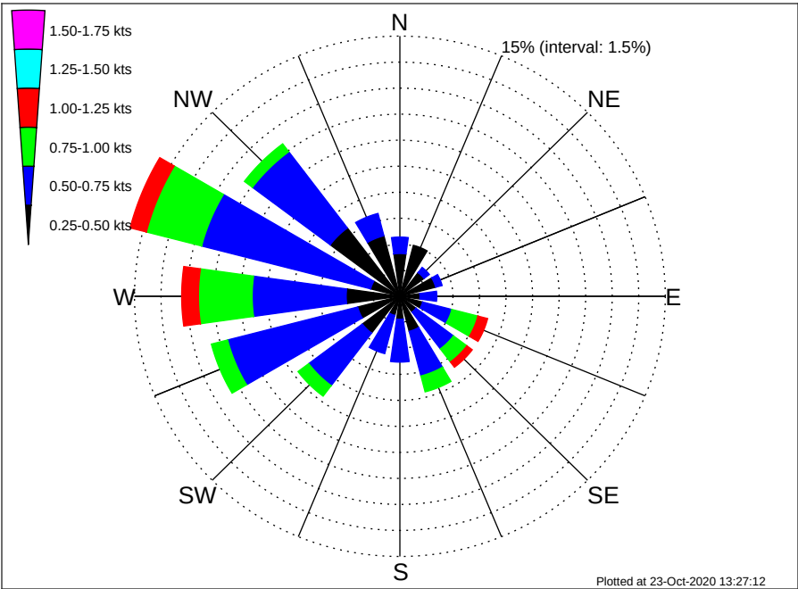
SpaceX GOM Launch Platform Climatological Surface Current Rose for January: 1995 - 2012
