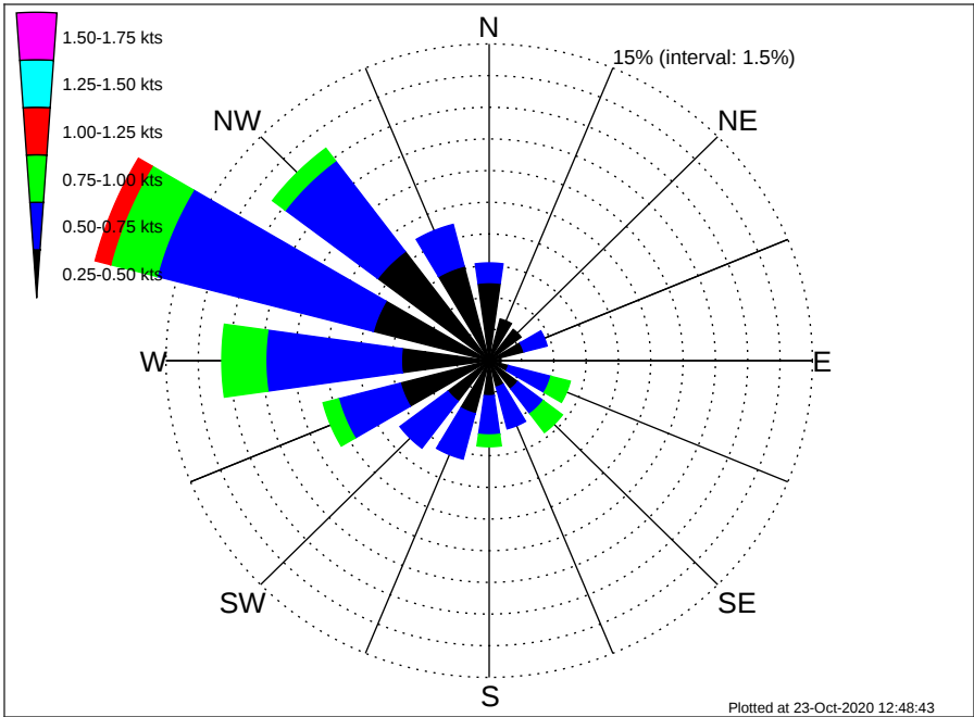
SpaceX GOM Launch Platform Climatological Surface Current Rose for November: 1995 - 2012
