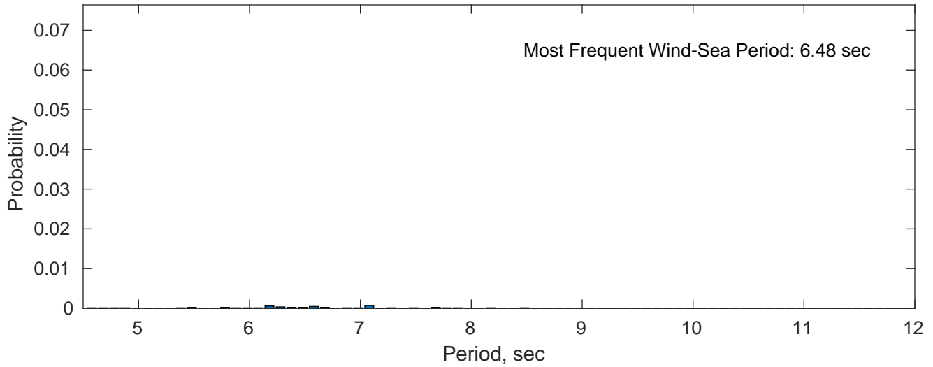
Wind-Sea: 0.53%
