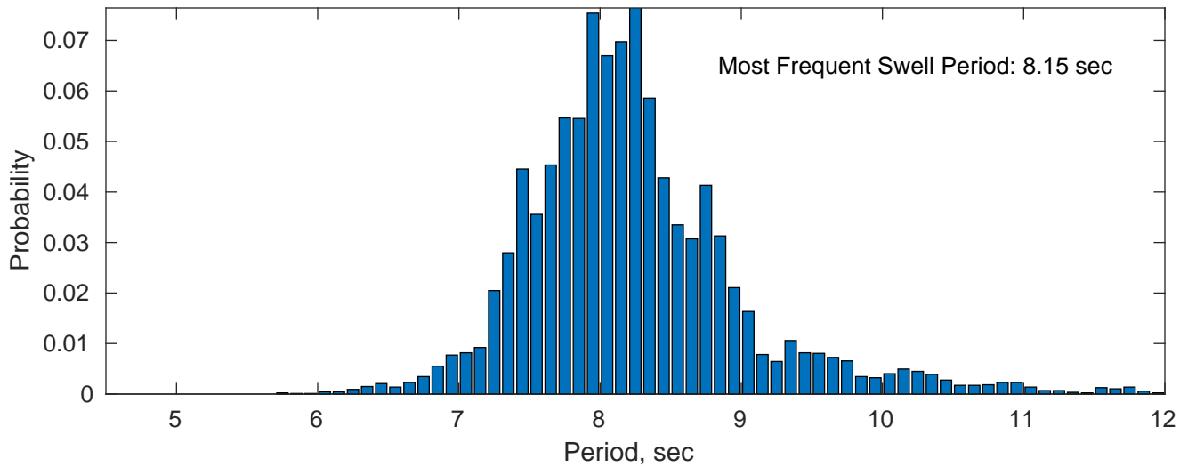
Swell: 99.47%
