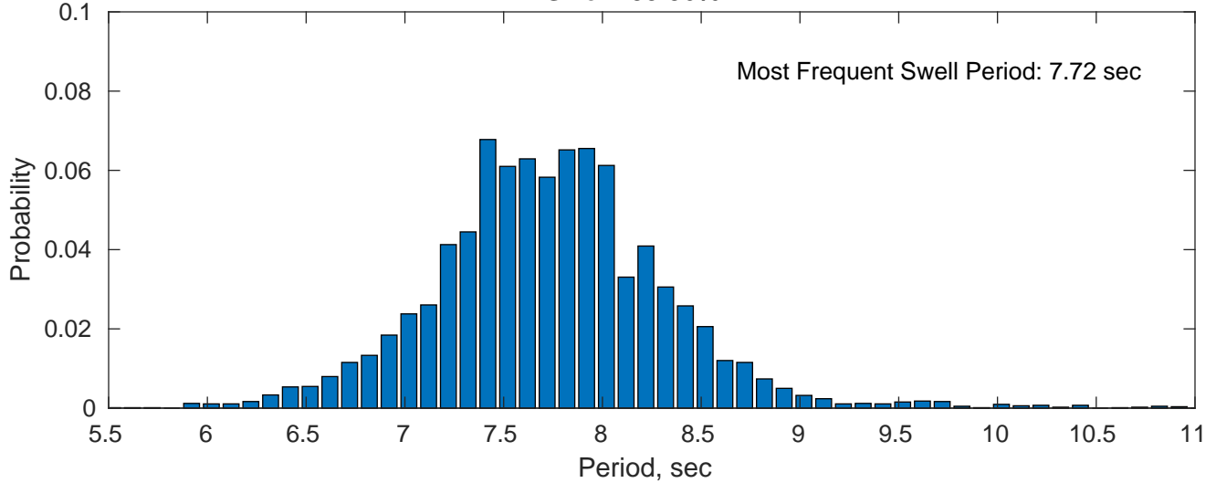
Swell: 85.86%
