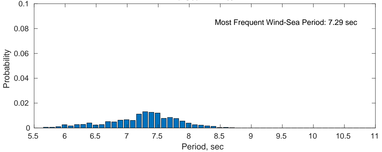
Wind-Sea: 14.14%
