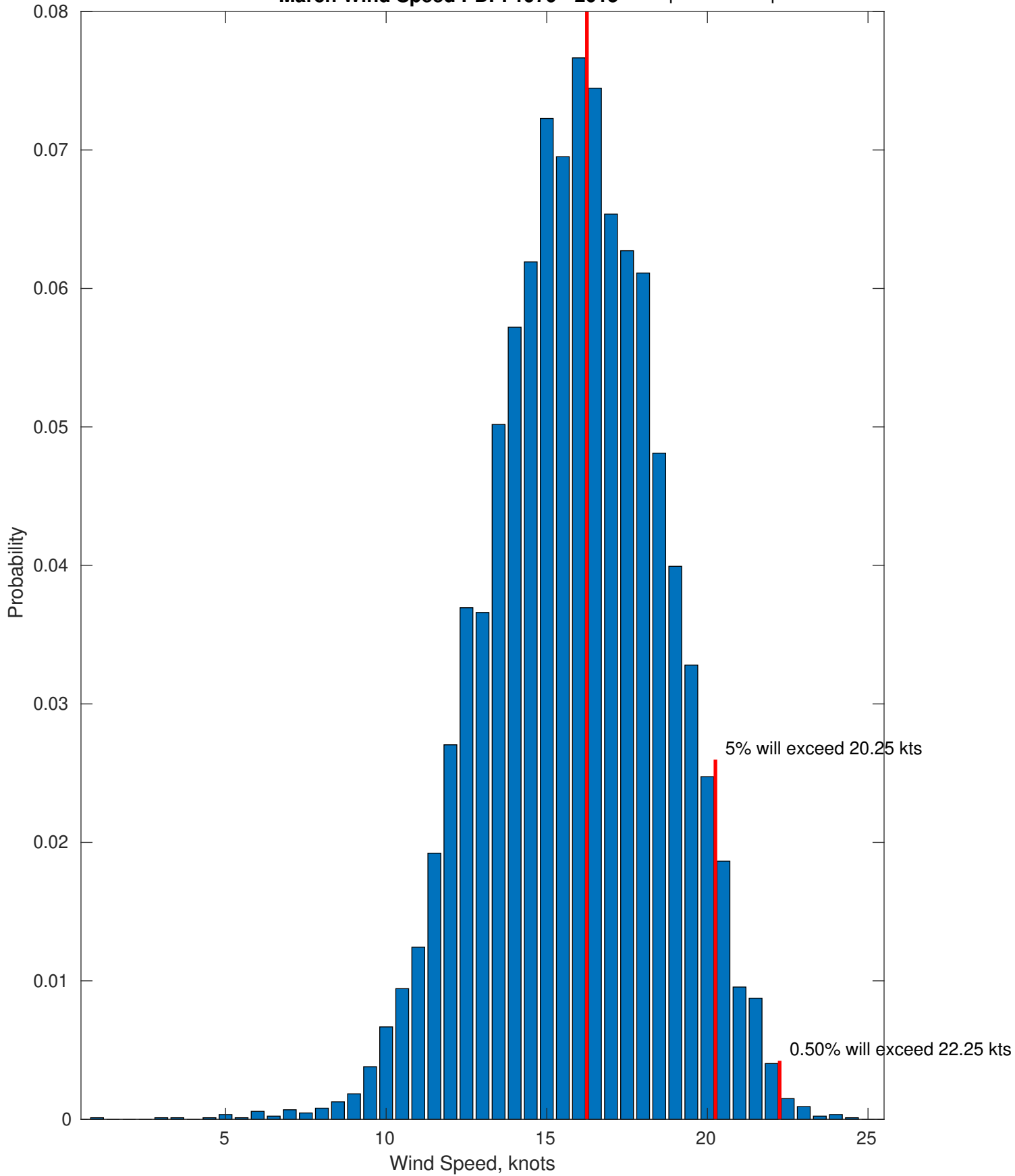
March Wind Speed PDF: 1979 - 2016 Most Frequent Wind Speed: 16.25 kts
