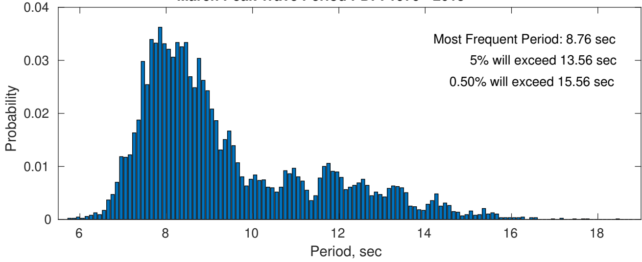
March Peak Wave Period PDF: 1979 - 2015
