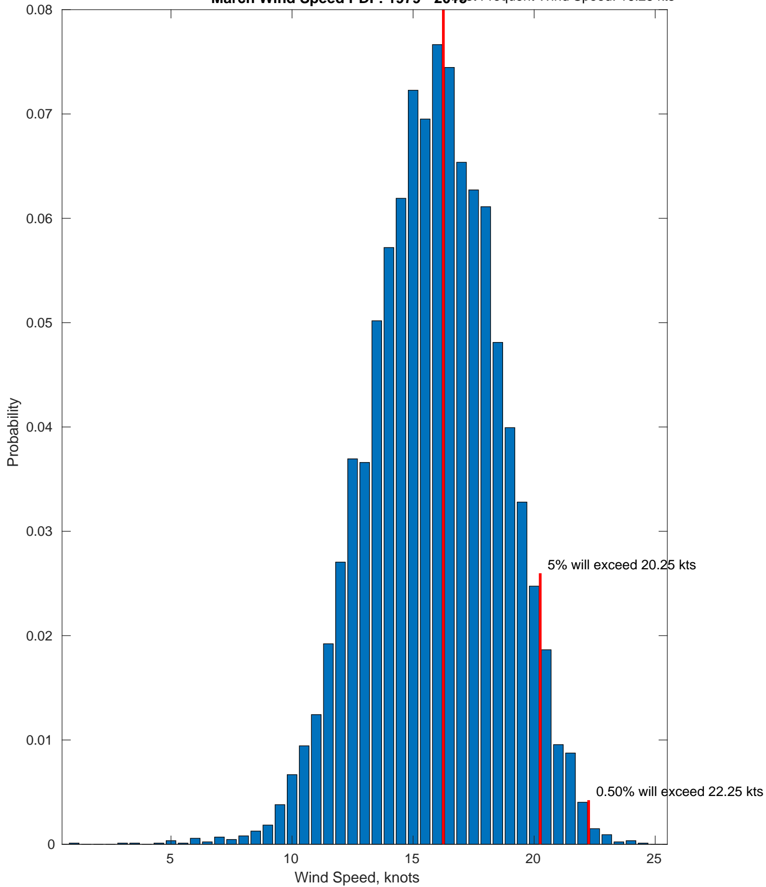
March Wind Speed PDF: 1979 - 2019 Most Frequent Wind Speed: 16.25 kts
