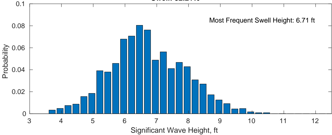
Swell: 82.21%
