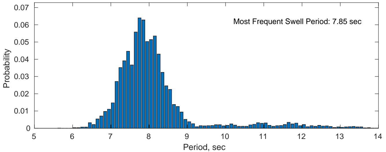
Swell: 82.21%
