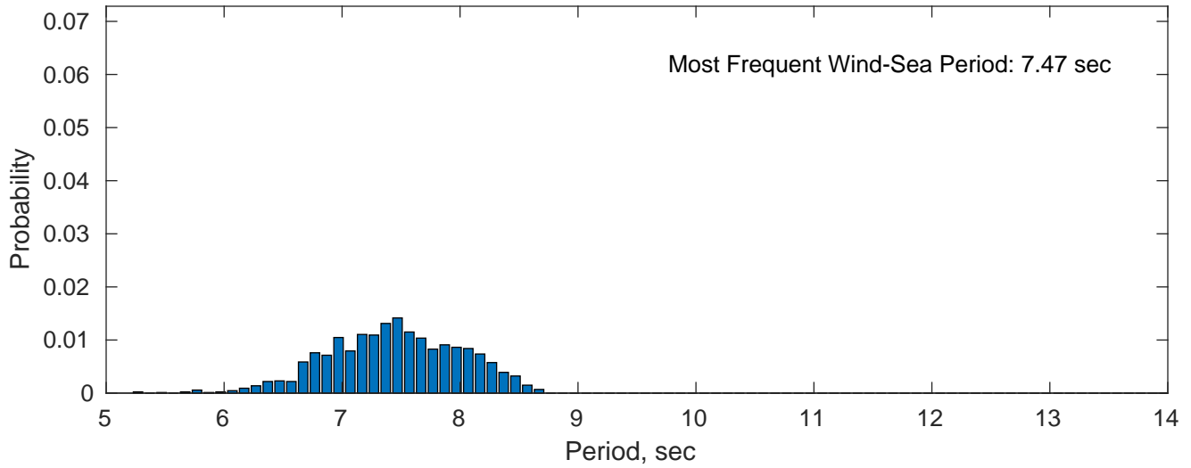
Wind-Sea: 17.79%
