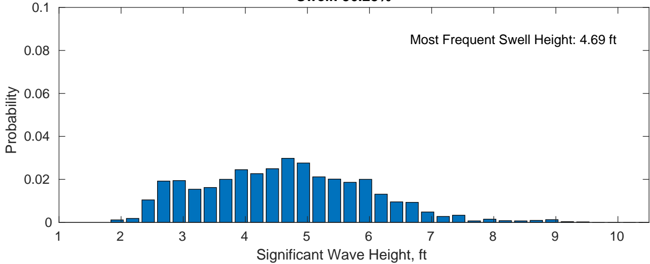
Swell: 36.28%
