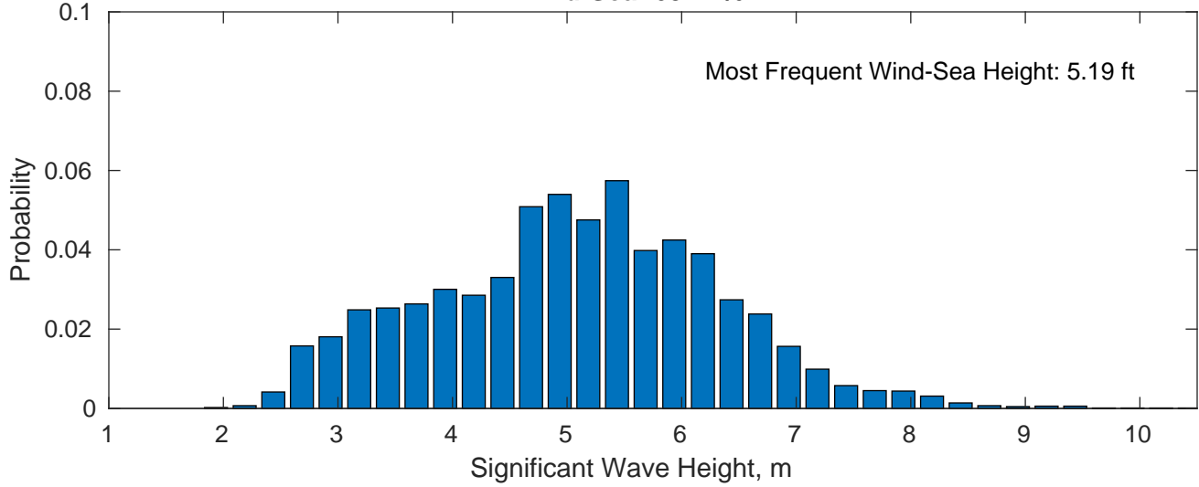
Wind-Sea: 63.72%
