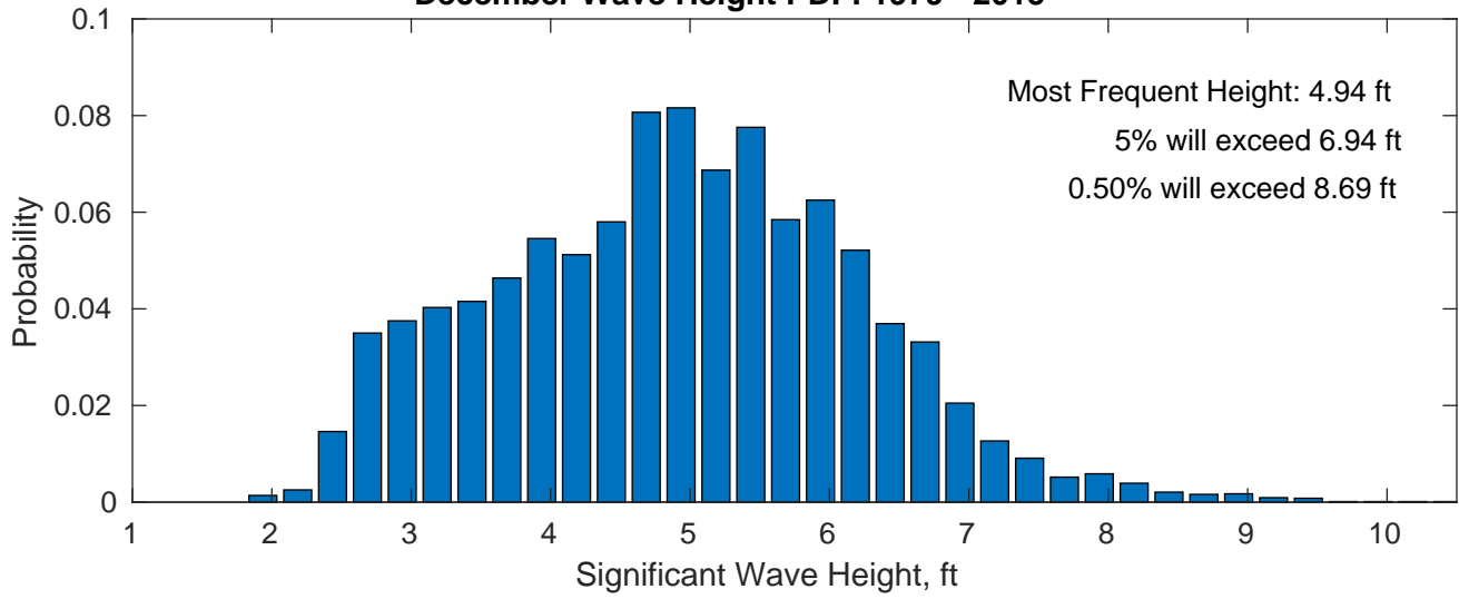
December Wave Height PDF: 1979 - 2015
