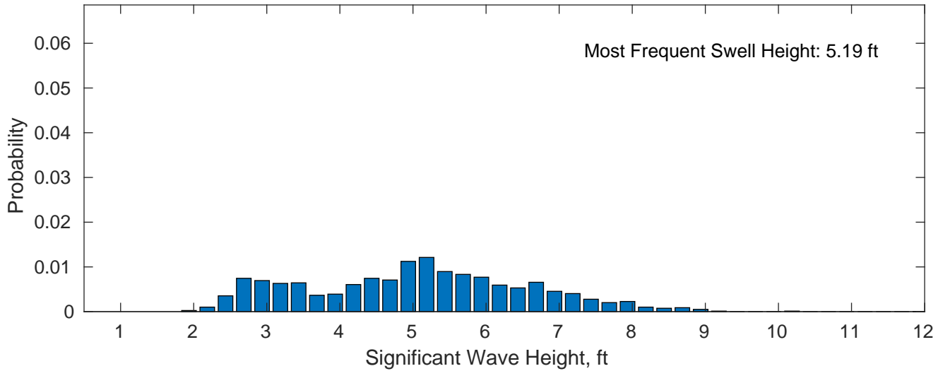
Swell: 14.53%
