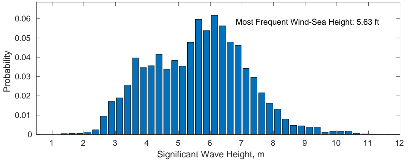
Wind-Sea: 85.47%
