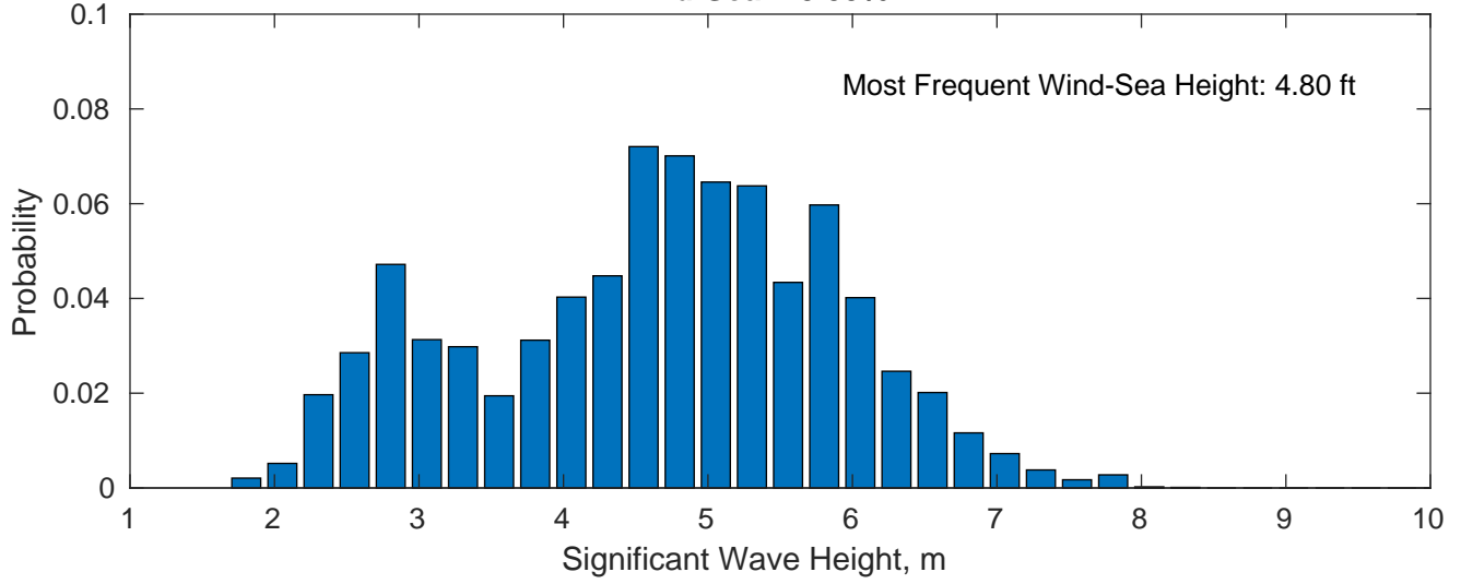
Wind-Sea: 78.55%
