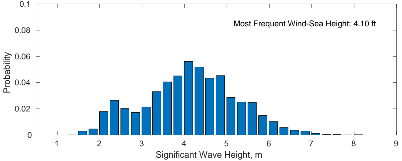
Wind-Sea: 54.51%
