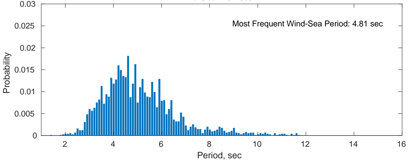
Wind-Sea: 43.20%
