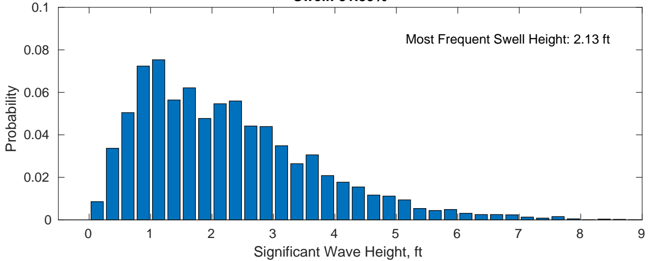
Swell: 81.39%
