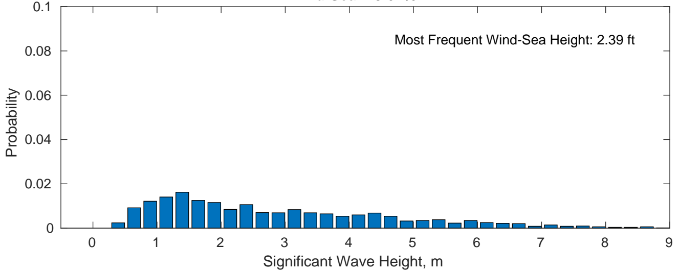
Wind-Sea: 18.61%
