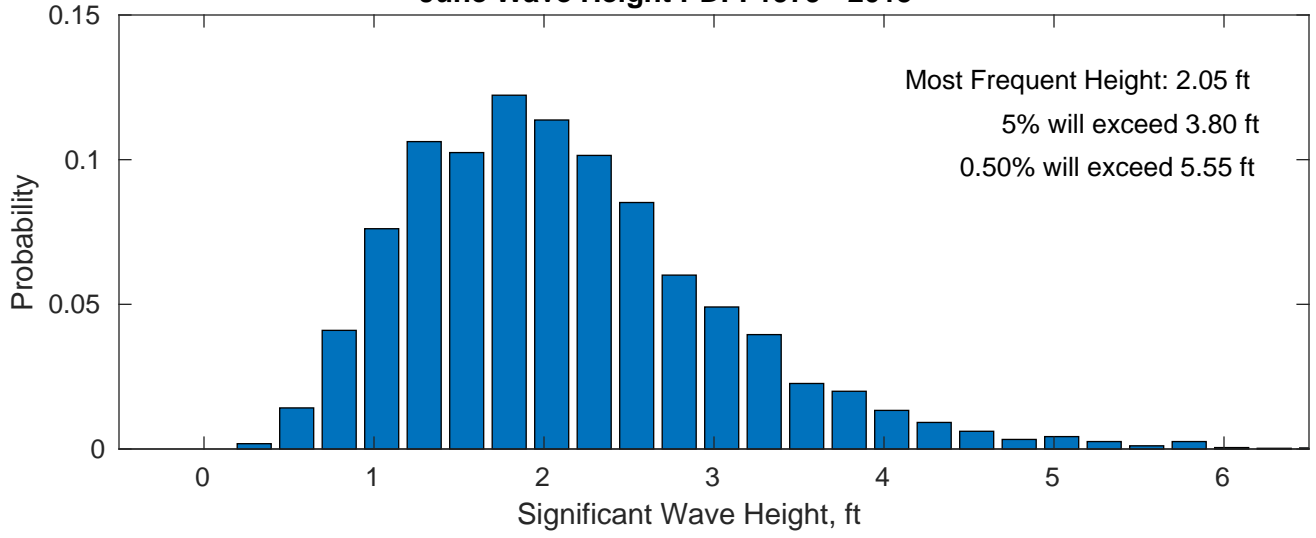
Wind-Sea: 6.40%
