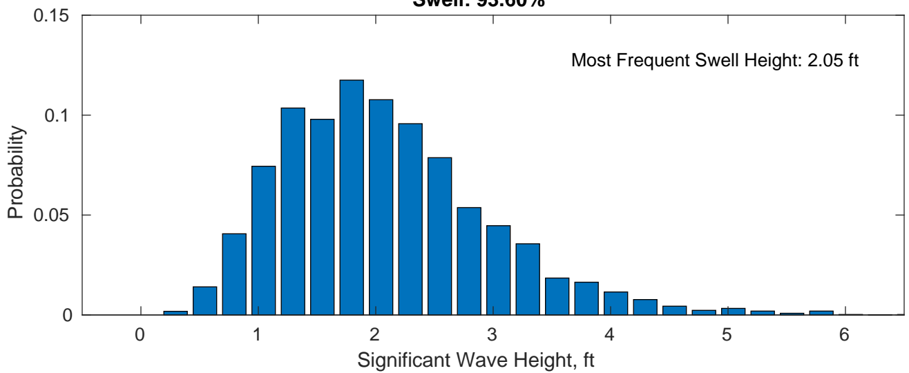
Swell: 93.60%
