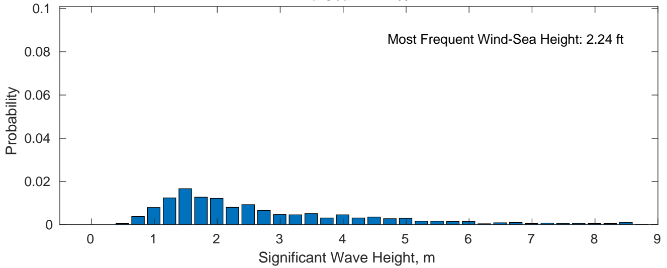
Wind-Sea: 14.12%
