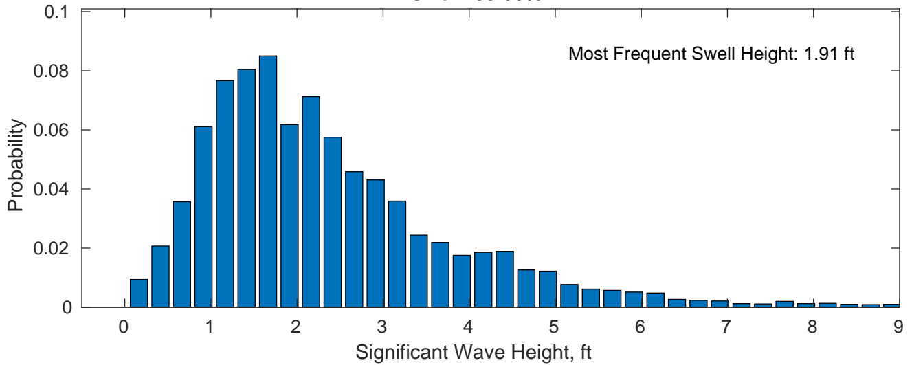
Swell: 85.88%
