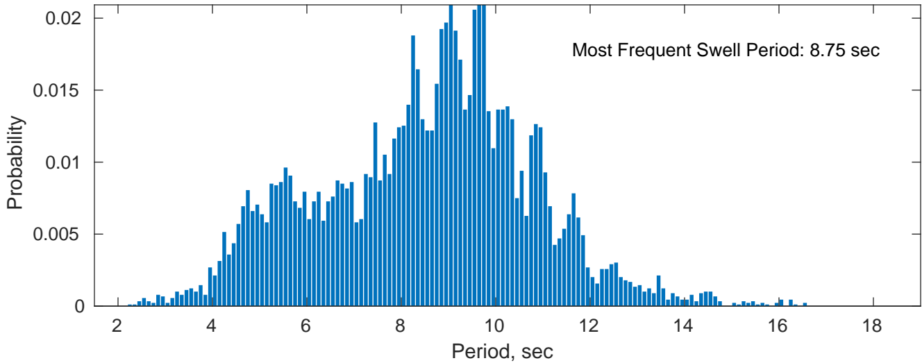
Swell: 85.88%
