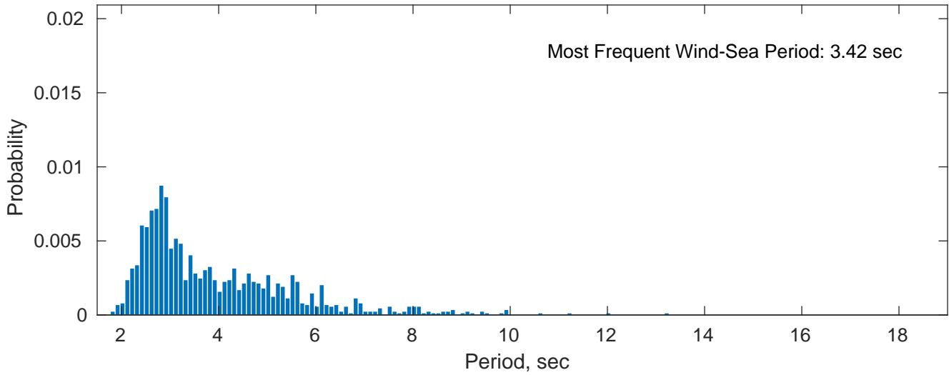
Wind-Sea: 14.12%
