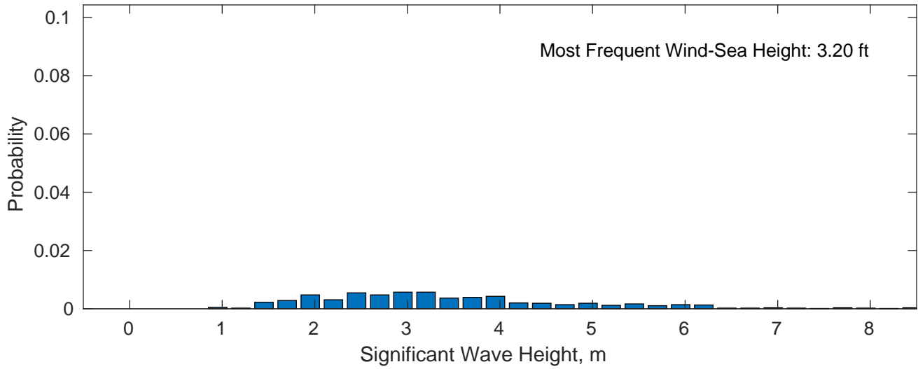
Wind-Sea: 6.59%
