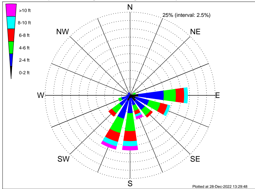
VNE 522 ECR Midpoint Climatological WaveHeight Rose for April: 1979 - 2015
