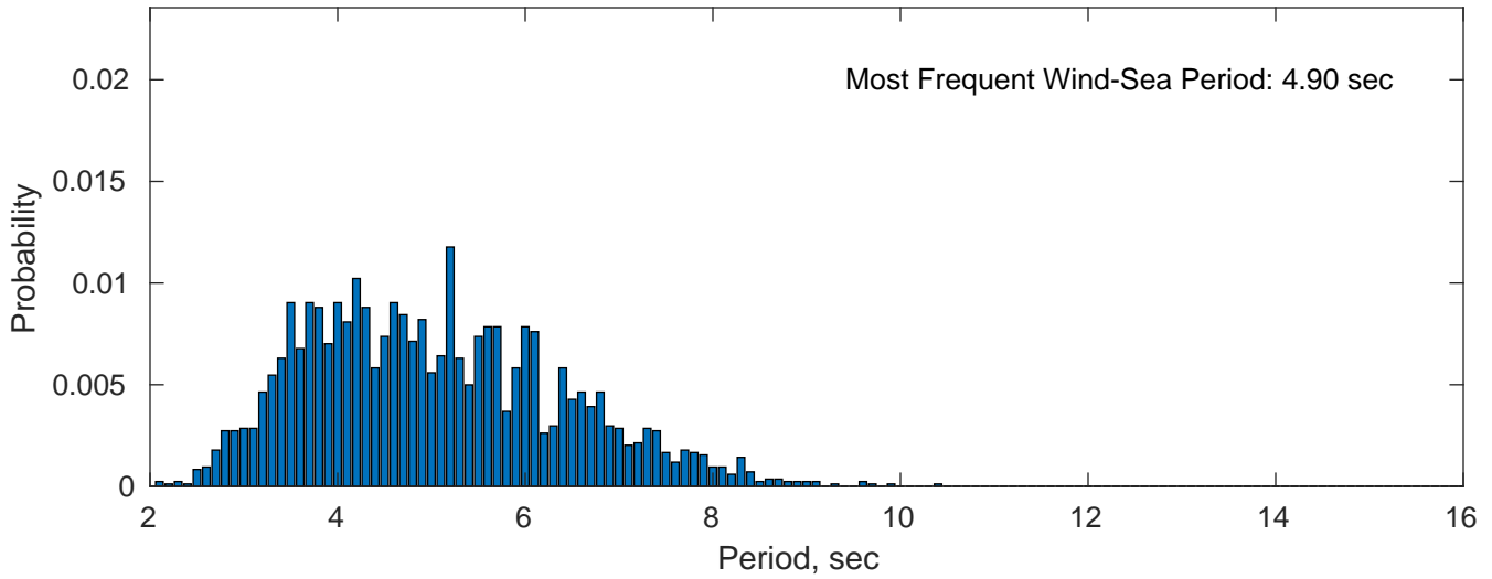
Wind-Sea: 29.74%
