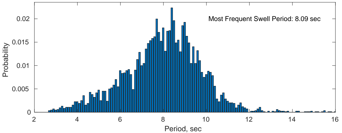
Swell: 70.26%
