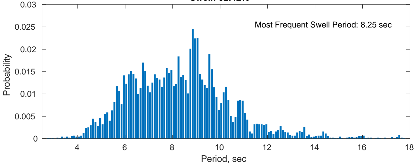
Swell: 82.42%
