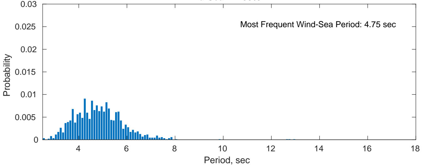
Wind-Sea: 17.58%
