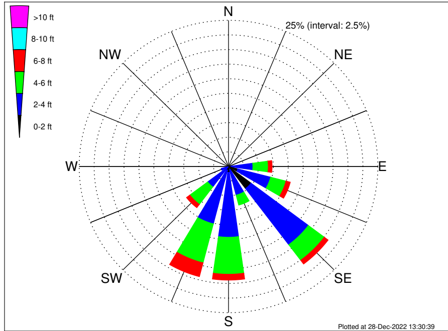
VNE 522 ECR Midpoint Climatological WaveHeight Rose for June: 1979 - 2015
