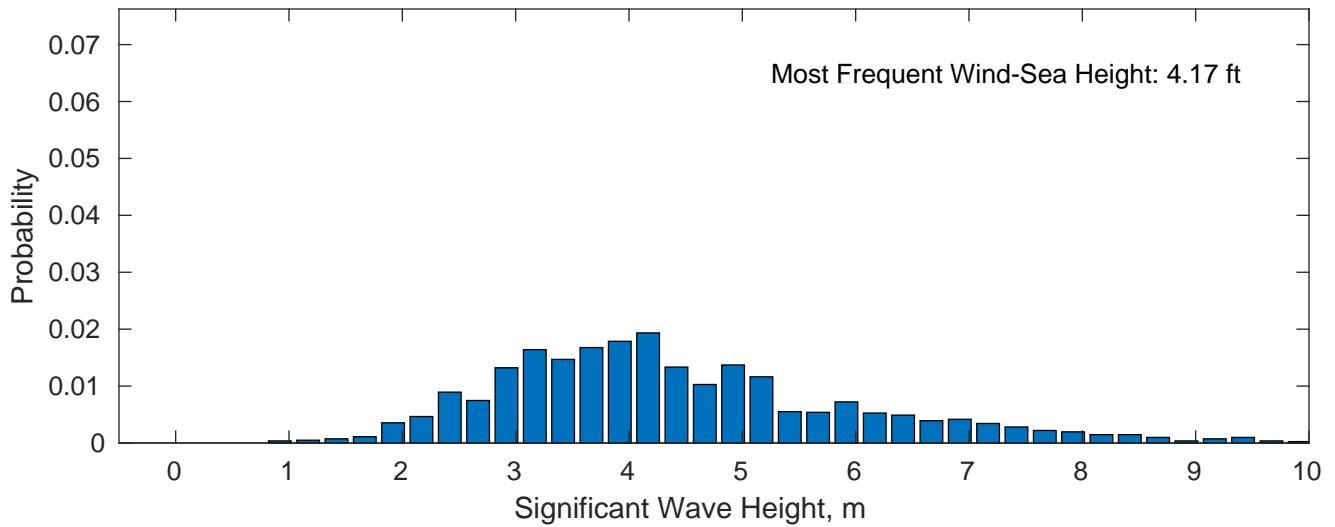
Wind-Sea: 22.86%
