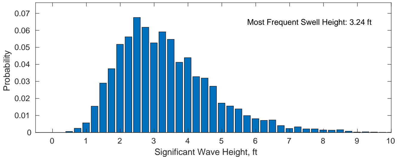
Swell: 77.14%
