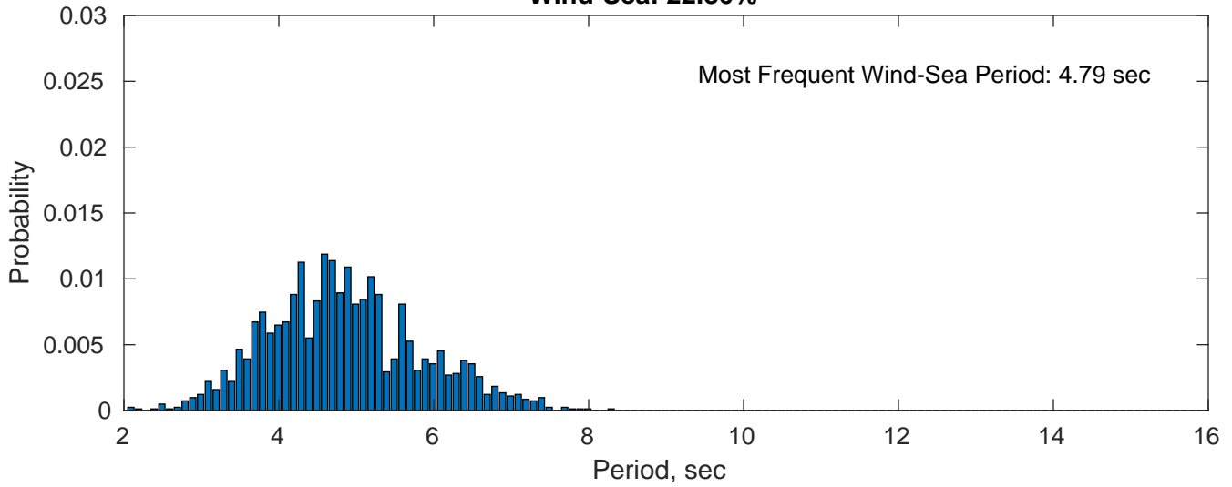
Wind-Sea: 22.86%
