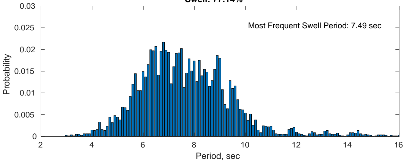
Swell: 77.14%
