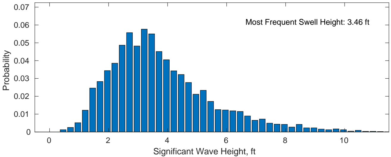
Swell: 75.91%
