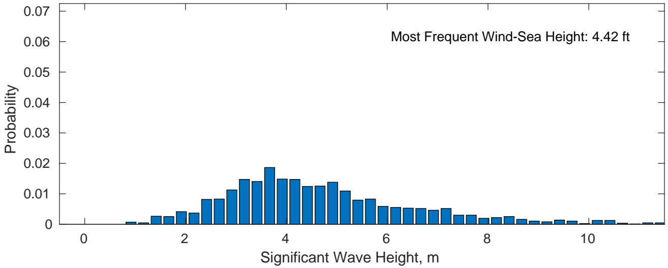
Wind-Sea: 24.09%
