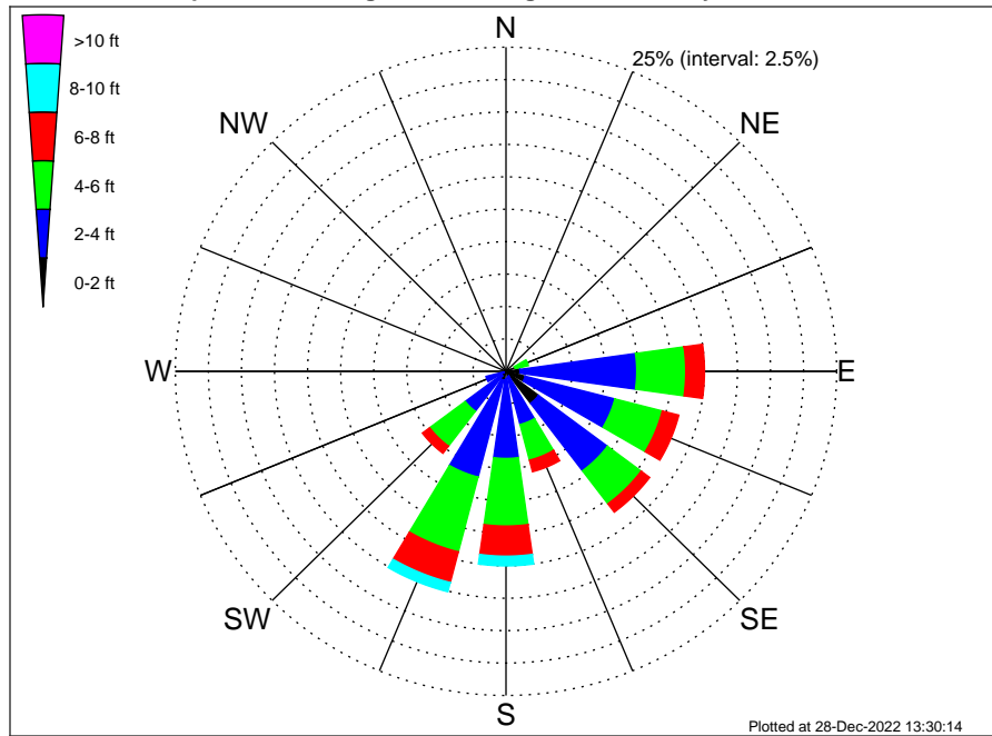
VNE 522 ECR Midpoint Climatological WaveHeight Rose for May: 1979 - 2015
