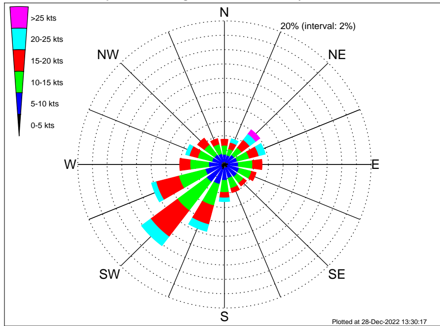
VNE 522 ECR Midpoint Climatological Wind Rose for May: 1979 - 2015
