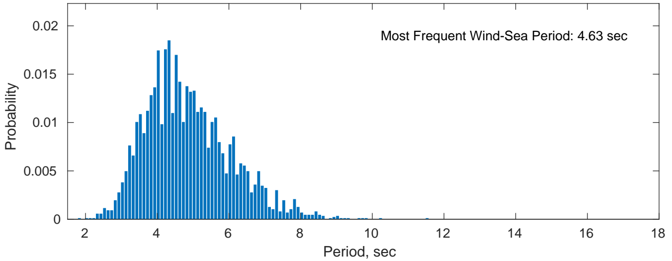
Wind-Sea: 41.08%
