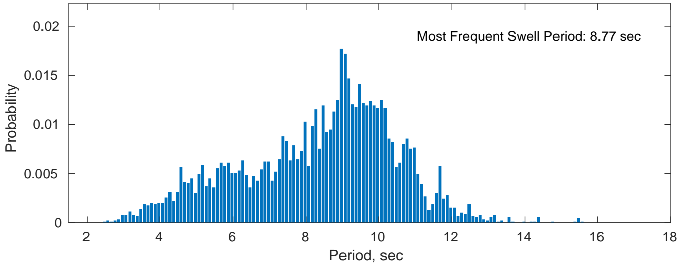
Swell: 58.92%
