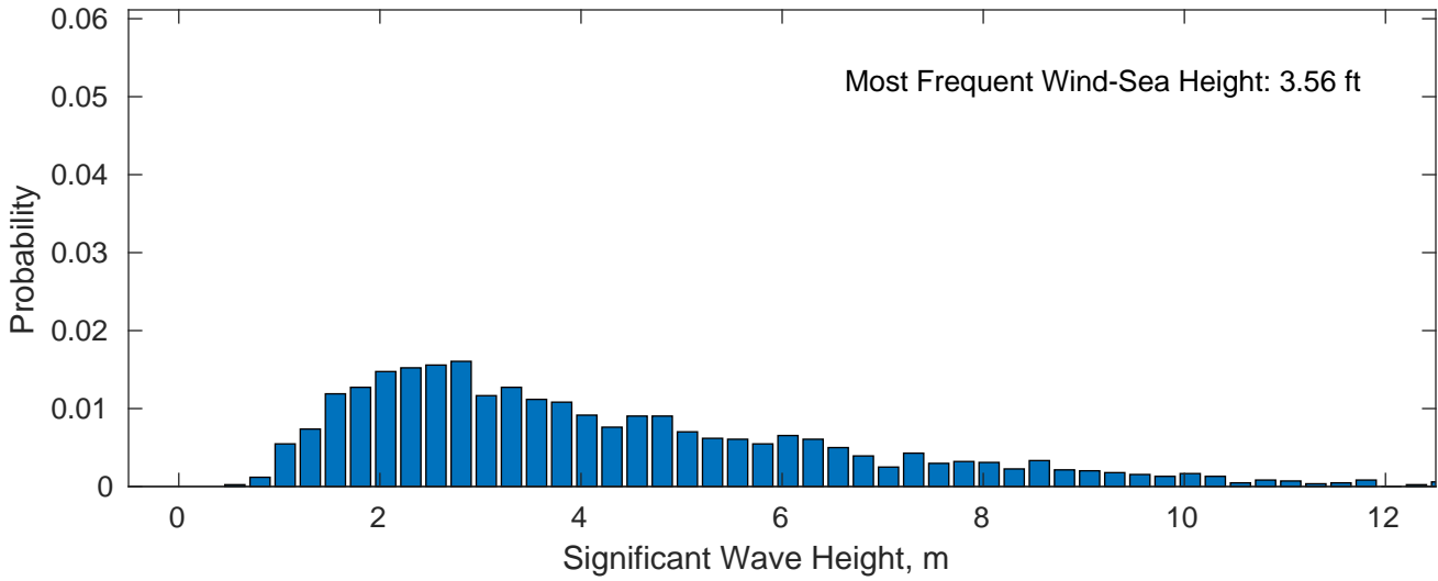
Wind-Sea: 26.67%
