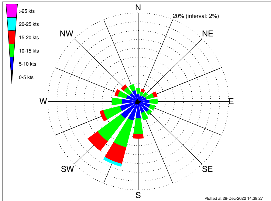
VNE 544 ECR1 Midpoint Climatological Wind Rose for June: 1979 - 2015
