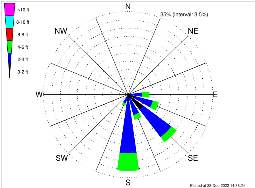
VNE 544 ECR1 Midpoint Climatological WaveHeight Rose for June: 1979 - 2015
