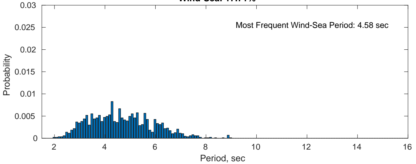
Wind-Sea: 17.71%
