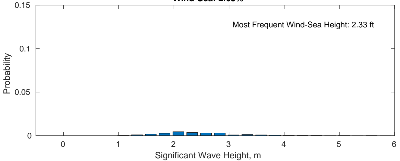
Wind-Sea: 2.65%
