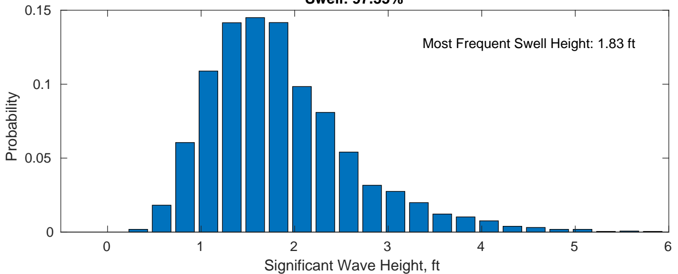
Swell: 97.35%
