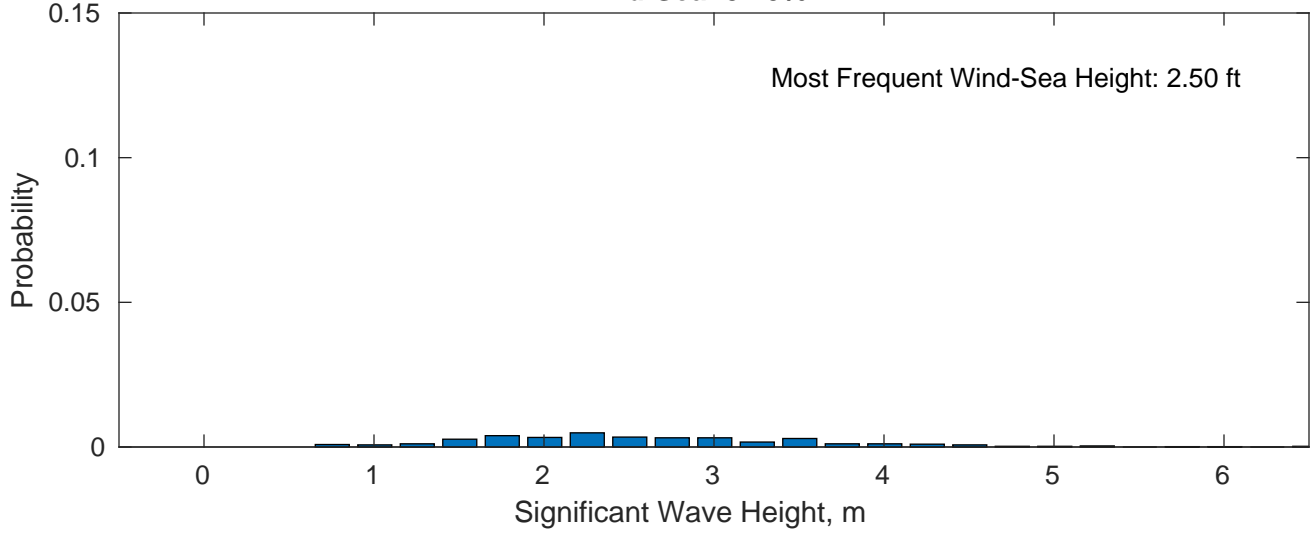
Wind-Sea: 3.75%
