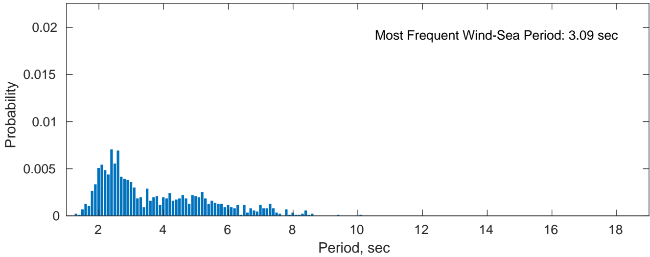
Wind-Sea: 13.25%
