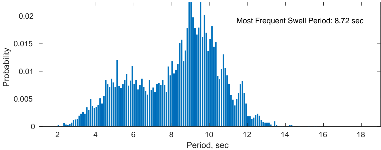
Swell: 86.75%
