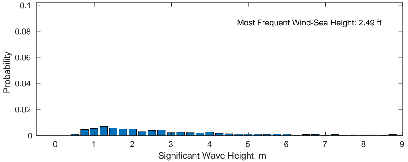
Wind-Sea: 7.79%
