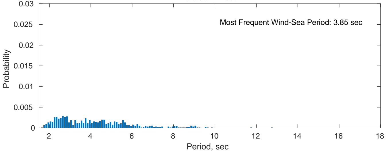
Wind-Sea: 7.79%
