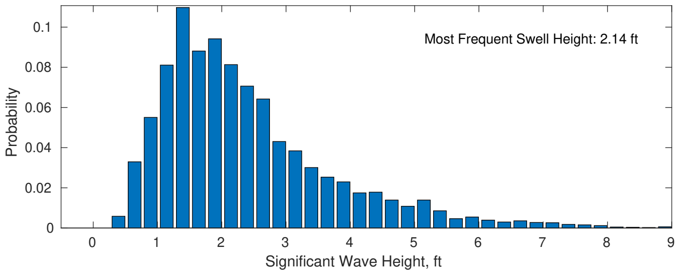
Swell: 95.98%
