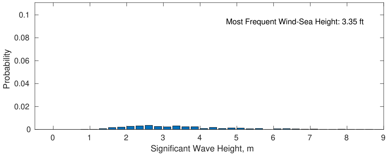
Wind-Sea: 4.02%
