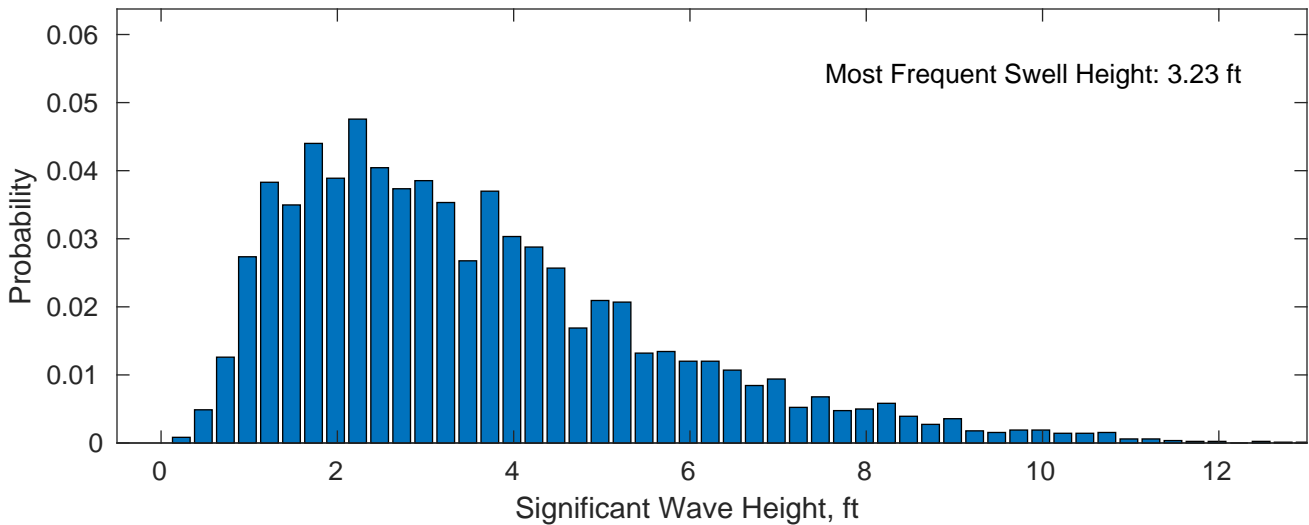
Swell: 73.94%
