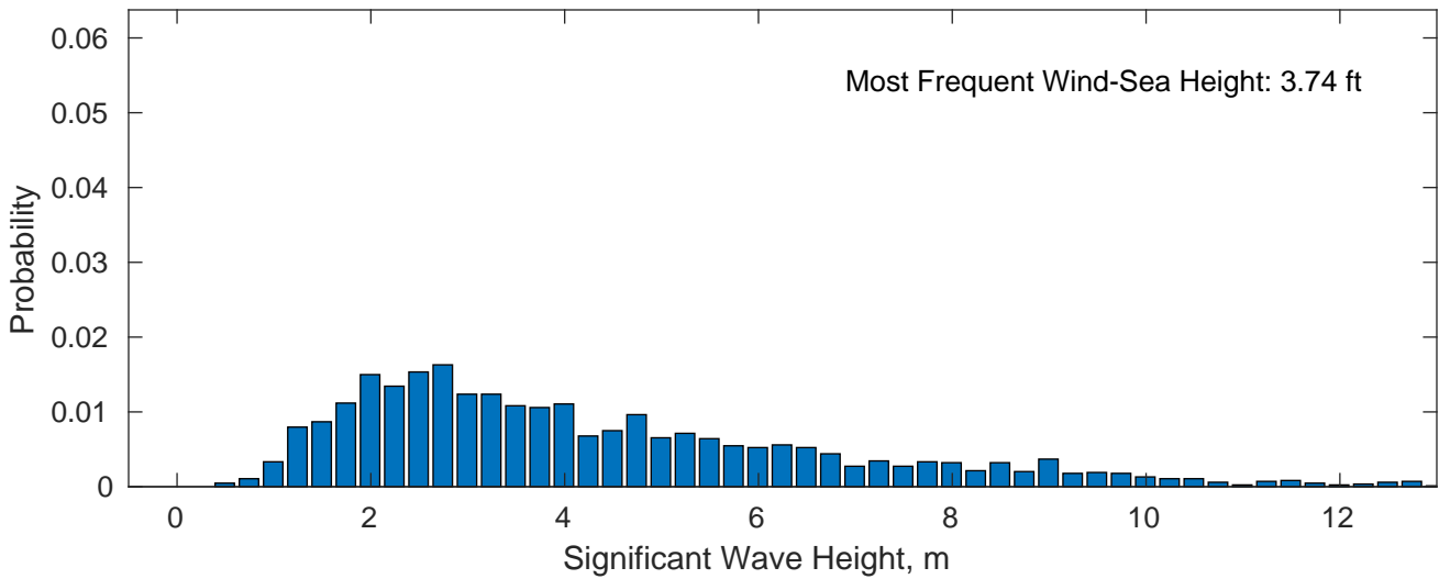
Wind-Sea: 26.06%
