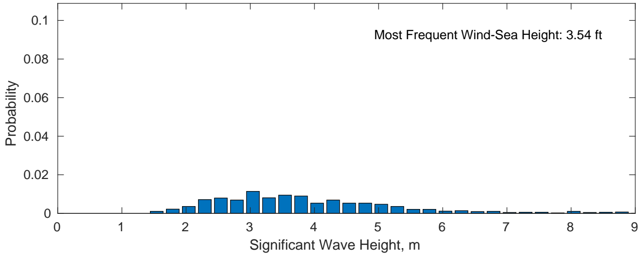
Wind-Sea: 11.37%
