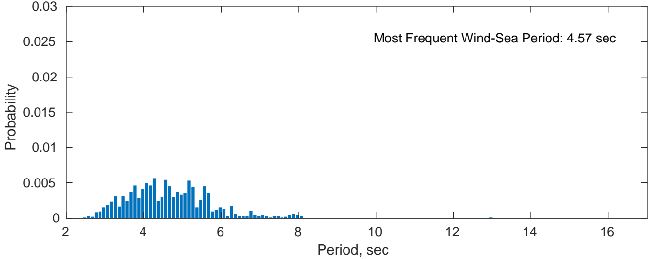
Wind-Sea: 11.37%
