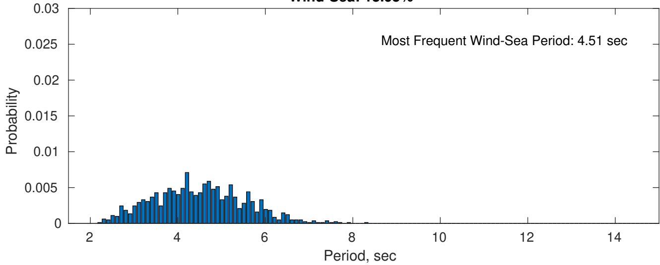
Wind-Sea: 13.95%
