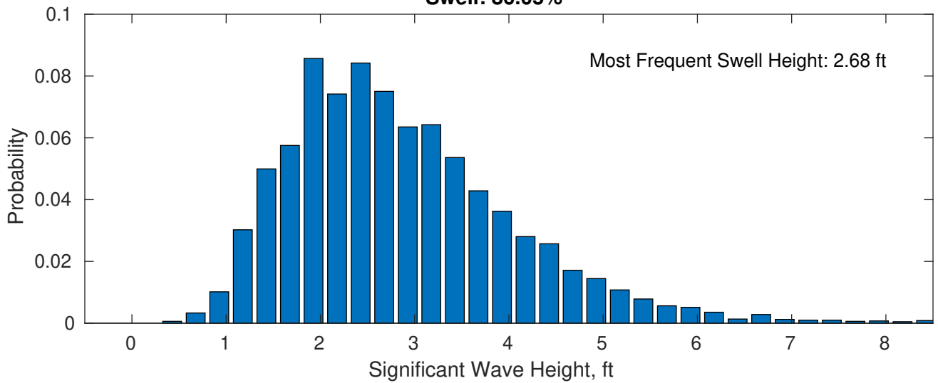
Swell: 86.05%
