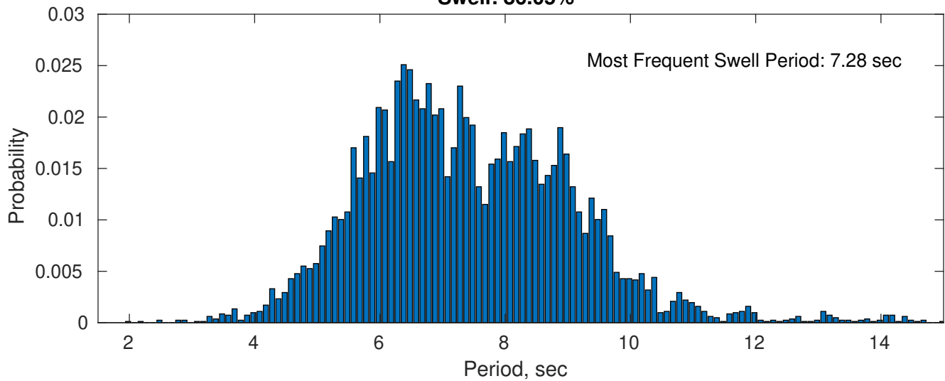
Swell: 86.05%
