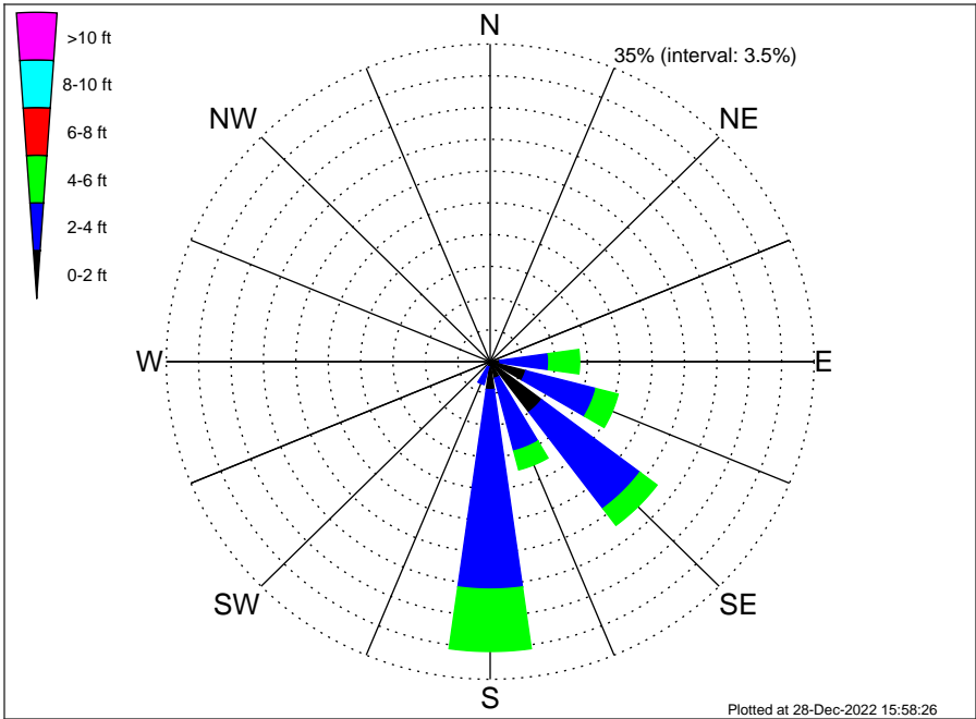
VNE 544 ECR2 Midpoint Climatological WaveHeight Rose for June: 1979 - 2015
