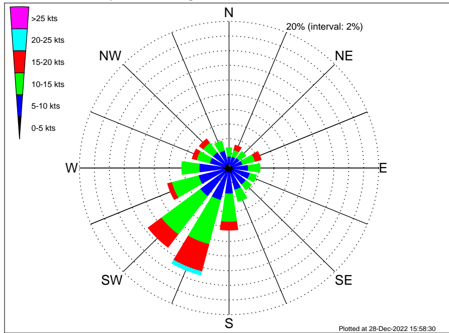
VNE 544 ECR2 Midpoint Climatological Wind Rose for June: 1979 - 2015
