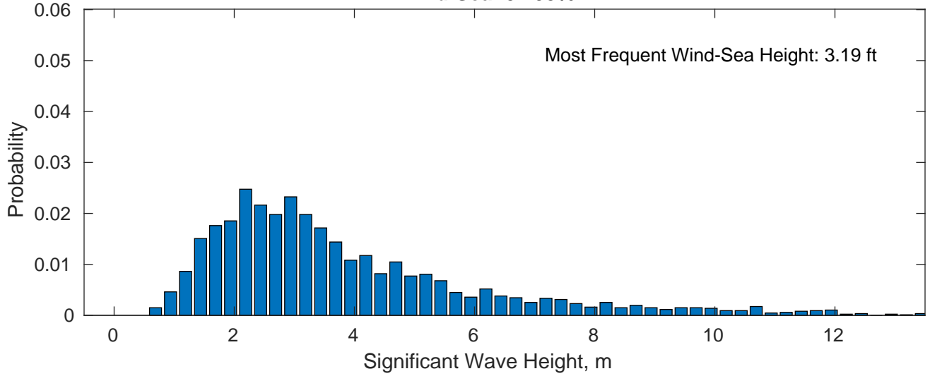
Wind-Sea: 32.93%
