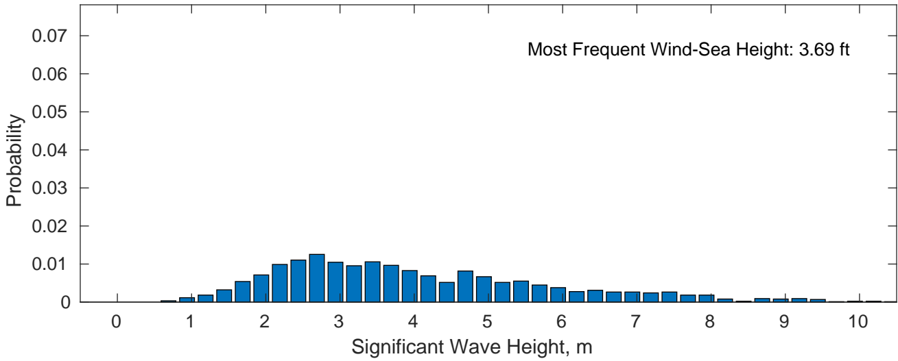
Wind-Sea: 17.38%
