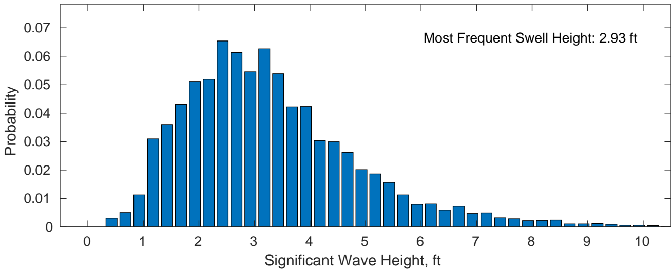
Swell: 82.62%
