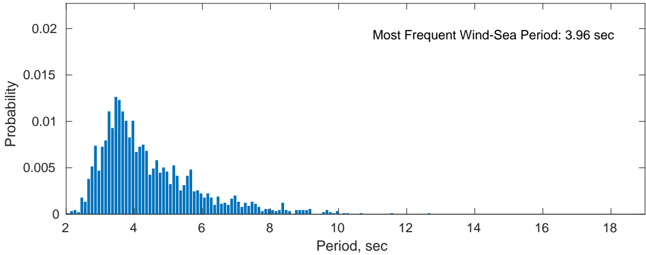
Wind-Sea: 24.95%
