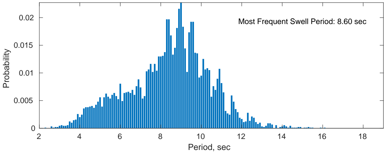
Swell: 75.05%
