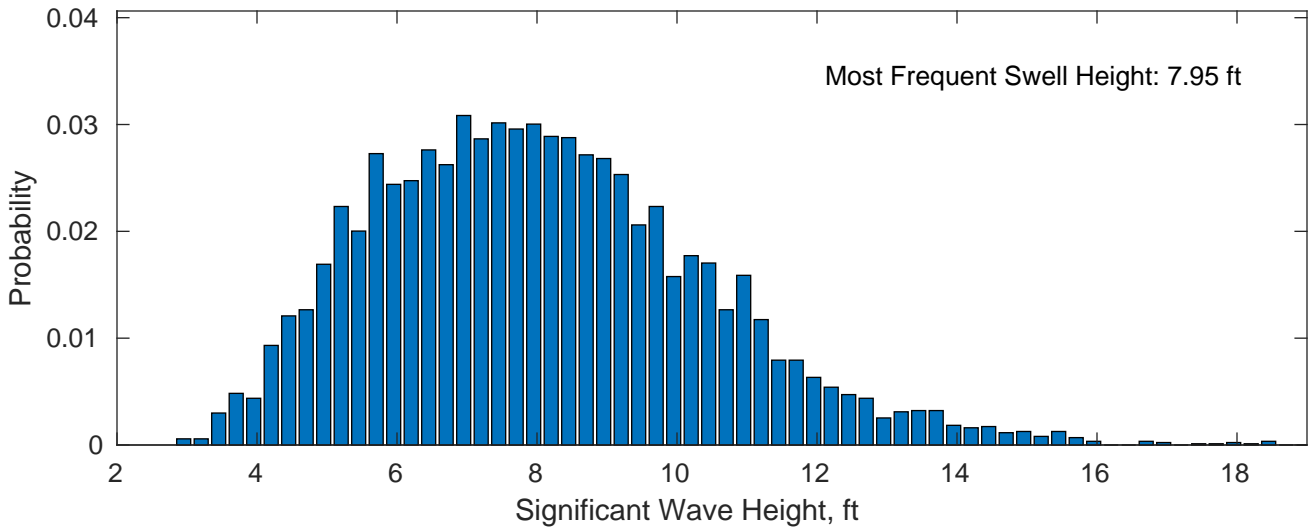
Swell: 71.79%
