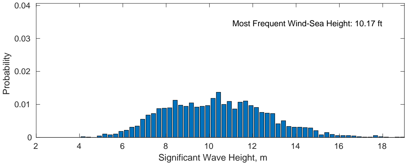
Wind-Sea: 28.21%
