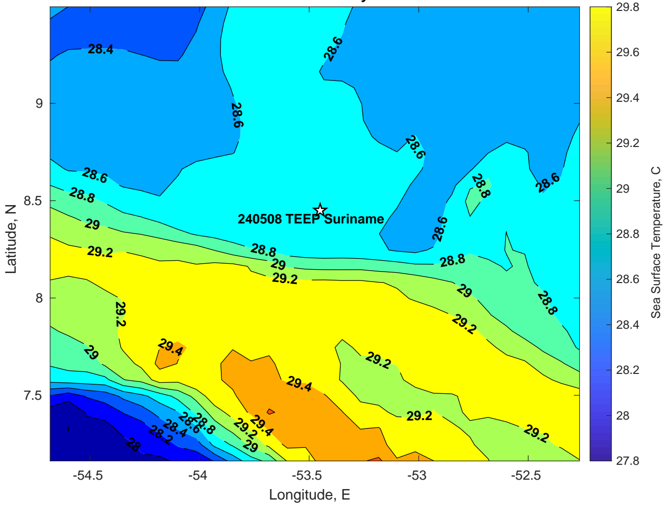
SST for 240508 TEEP Suriname at 15-May-2024 00:00:00
