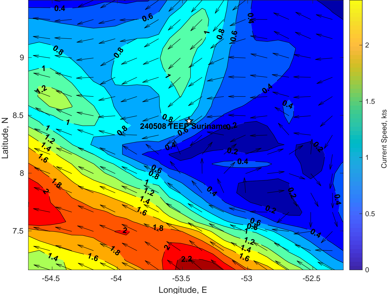
Surface Currents for 240508 TEEP Suriname at 15-May-2024 00:00:00
