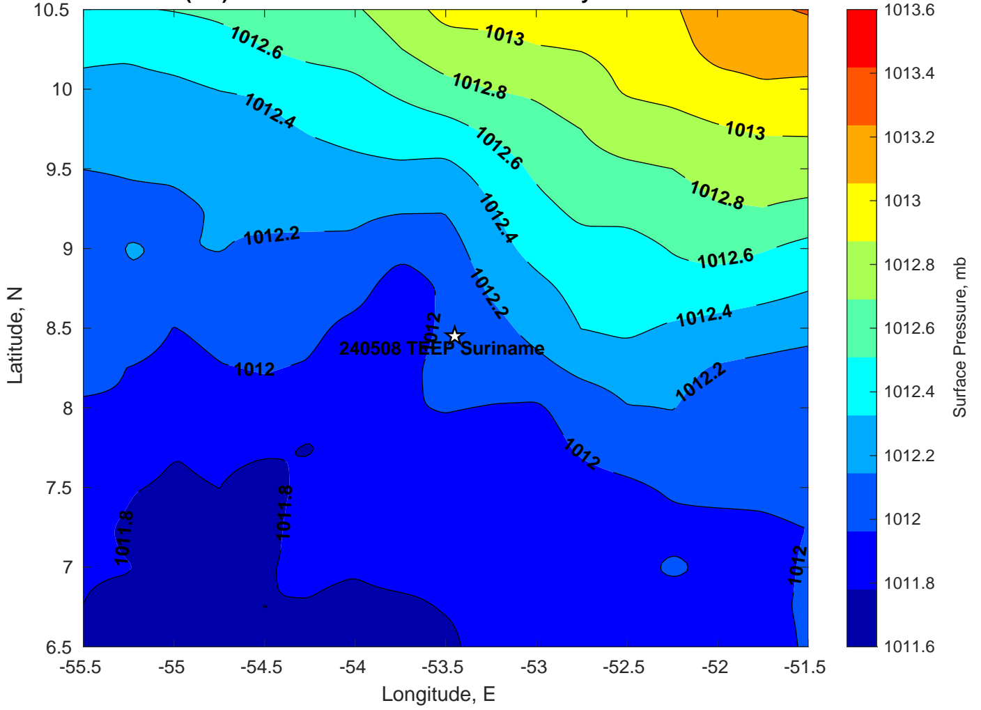
Surface Pressure (mb) for 240508 TEEP Suriname at 16-May-2024 12:00:00
